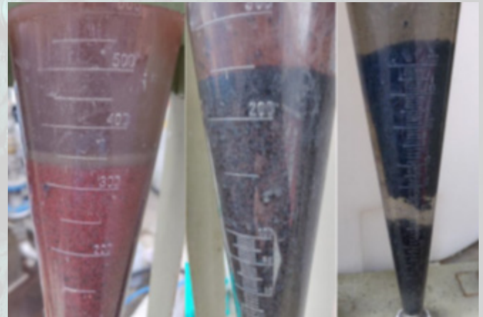
Figure 4 - Granular and Flocculent Biomass
